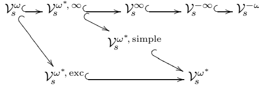
FIGURE 9.3. Subspaces of the principal series space \mathcal{V}_s .
