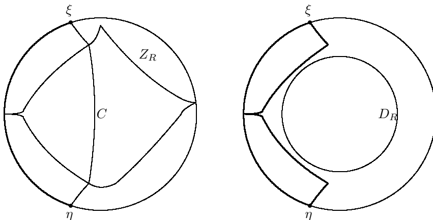
FIGURE 16.1. Proof of Lemma 16.5; illustrations.
