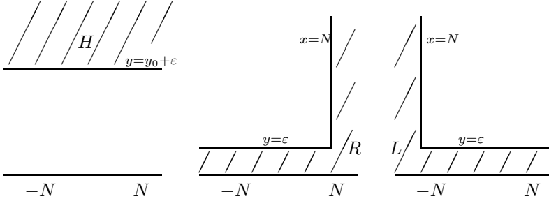
FIGURE 9.4. The regions H = \{z \in \mathfrak{H} : y > y_0 + \varepsilon\} , R = \{z \in \mathfrak{H} : x > N \text{ or } y < \varepsilon\} , and L = \{z \in \mathfrak{H} : x < -N \text{ or } y < \varepsilon\} .
