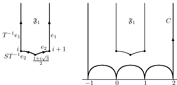
FIGURE 14.1. Fundamental domain \mathfrak{F}_1 for the modular group, and a 1-cycle around it.
