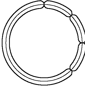
FIGURE 9.2. An excised neighborhood of \mathbb{S}^1 \setminus \{e^{-\pi i/4}, 1, e^{\pi i/4}, i\} for the disk model.
