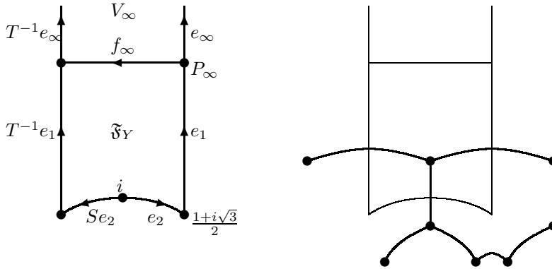
FIGURE 11.1. Modular group, parts of tessellations of type Fd (left) and Dir (right).
