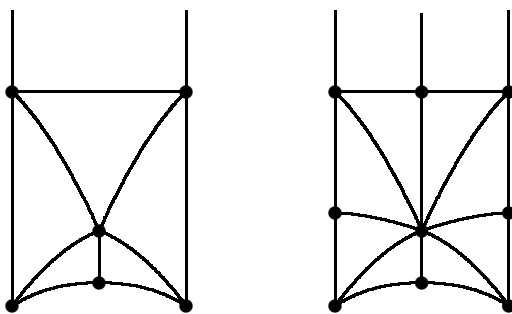
FIGURE 11.2. Modular group, part of tessellations of type Mix (left) and Mix' (right).
