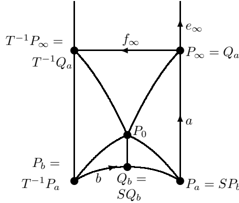
FIGURE 19.1. The points P_e and Q_e in the standard fundamental domain of the modular group.
