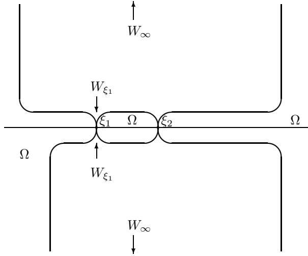
FIGURE 9.1. An excised neighborhood \Omega of \mathbb{P}_{\mathbb{R}}^1 \setminus \{\xi_1, \xi_2, \infty\} .
