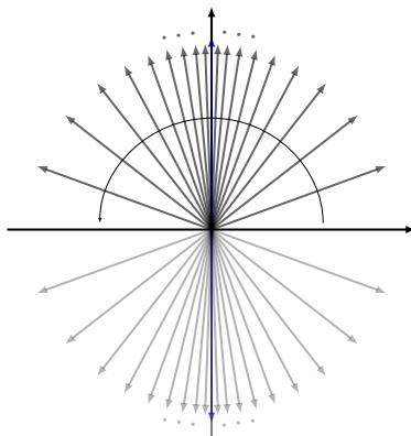
FIGURE 1. A peacock arrangement of Stokes rays in the complex Borel plane.
