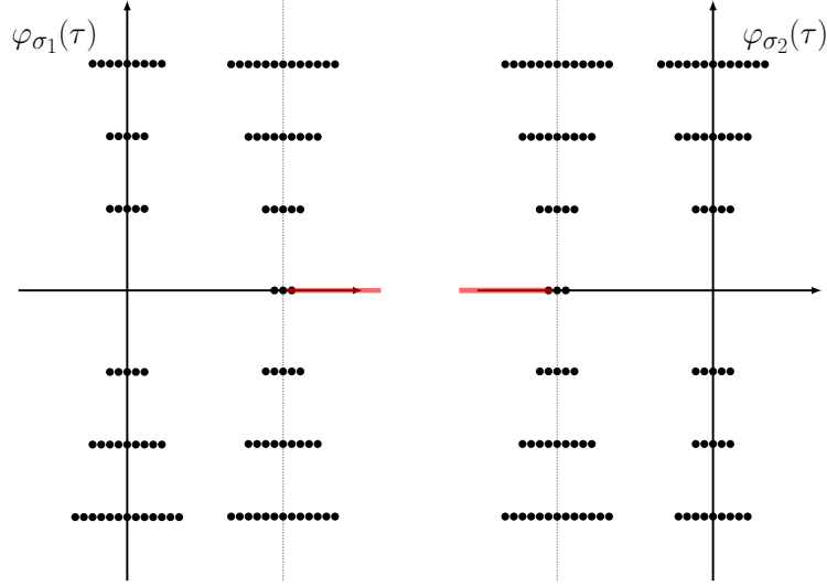
FIGURE 6. The singularities in the Borel plane for the series \varphi_{\sigma_j}(x; \tau) with j = 1, 2 of knot 4_1 where x is close to 1. The shortest vertical spacing between singularities is 2\pi i , and the horizontal spacing between neighboring singularities in each cluster is \log x .
