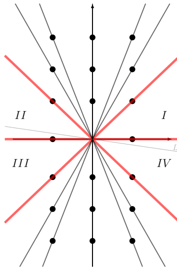
FIGURE 3. Four different sectors in the \tau -plane for \Phi(0; \tau) of knot \mathbf{4}_1 .
