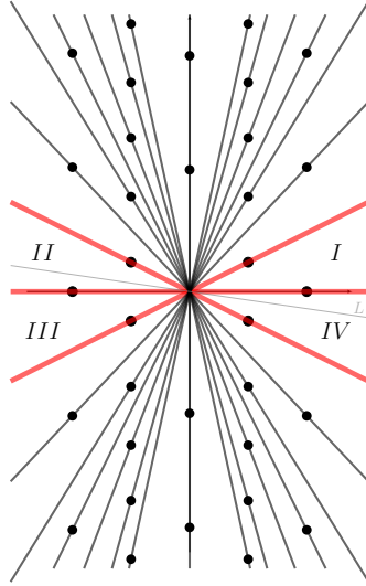
FIGURE 5. Four different sectors in the \tau -plane for \Phi(0; \tau) of knot \mathbf{5}_2 and the line L that divides the \tau -plane.
