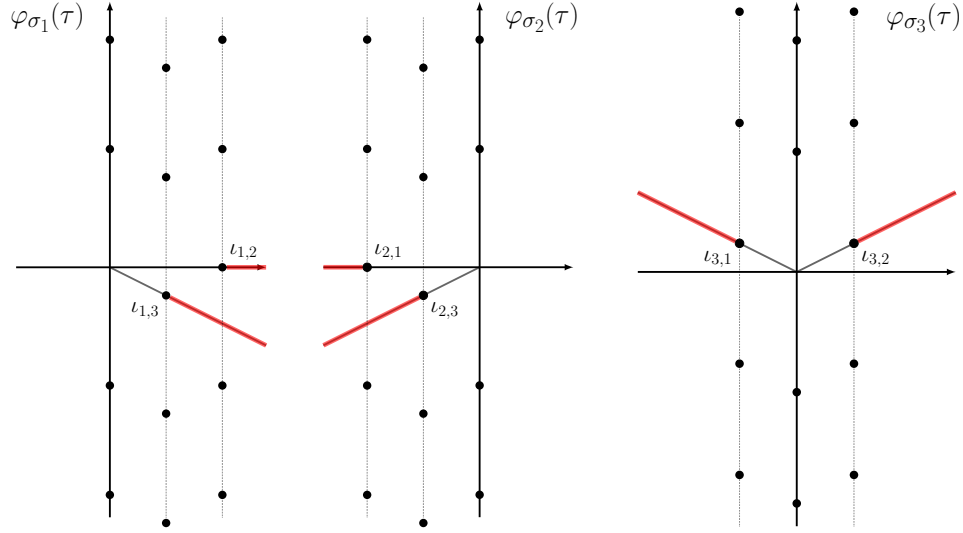
FIGURE 4. The singularities in the Borel plane for the series \varphi_{\sigma_j}(0; \tau) for j = 1, 2, 3 of knot \mathbf{5}_2 .
