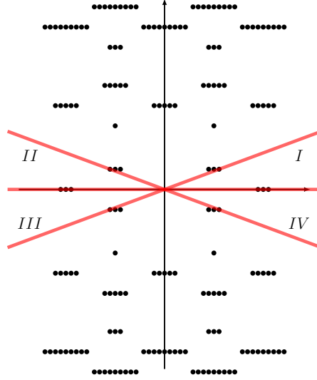
FIGURE 11. Four different sectors (and additional two auxiliary regions) in the \tau -plane for \Phi(u; \tau) of knot \mathbf{5}_2 with u close to zero.
