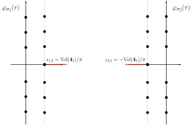
FIGURE 2. The singularities in the Borel plane for the series \varphi_{\sigma_j}(0; \tau) for j = 1, 2 of knot \mathbf{4}_1 .
