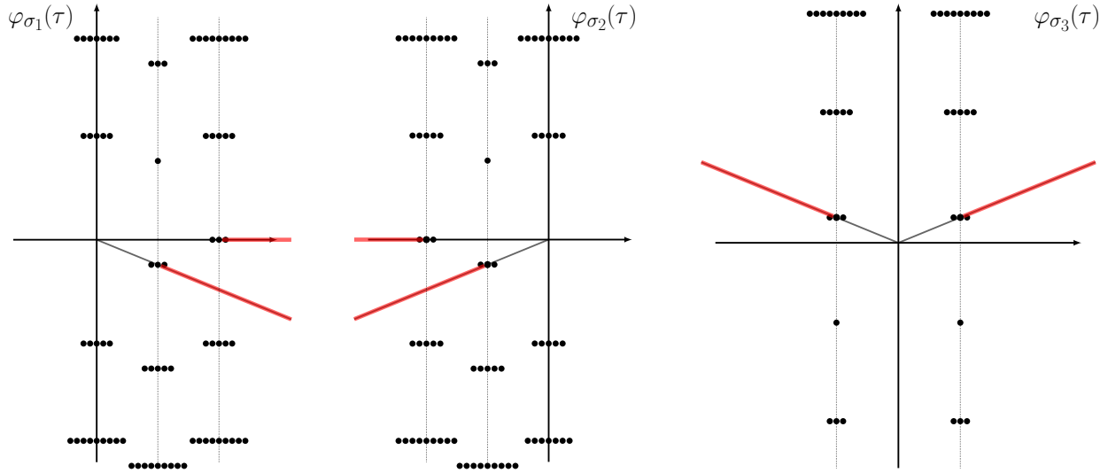
FIGURE 10. The singularities in the Borel plane for the series \varphi_{\sigma_j}(u; \tau) with j = 1, 2, 3 of knot \mathfrak{5}_2 where u is close to zero.
