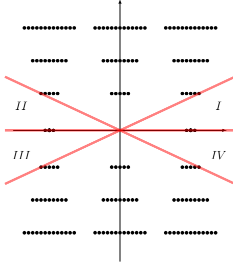
FIGURE 7. Four different sectors in the \tau -plane for \Phi(u; \tau) of knot 4_1 with u close to zero.
