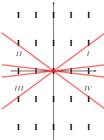
FIGURE 9. Four different sectors in the \tau -plane for \Phi(u; \tau) of knot 4_1 with x = e^{2\pi bu} in the first or the third interval of the positive axis.
