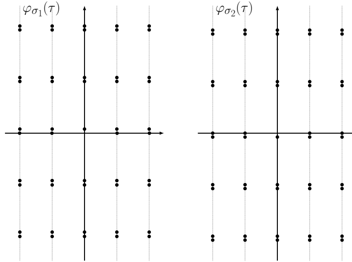
FIGURE 8. The singularities in the Borel plane for the series \varphi_{\sigma_j}(u; \tau) with j = 1, 2 of knot 4_1 for x = e^{2\pi b u} in the first or the third interval of the positive axis.
