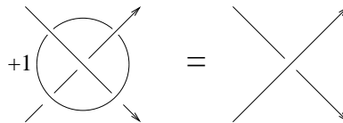
Figure 1. A crossing change can be achieved by surgery on a unit framed unknot.
