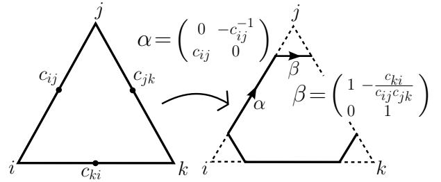
Figure 3. From Ptolemy assignments to natural cocycles.
