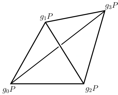
Figure 4. Decoration; equivariant assignment of cosets.
