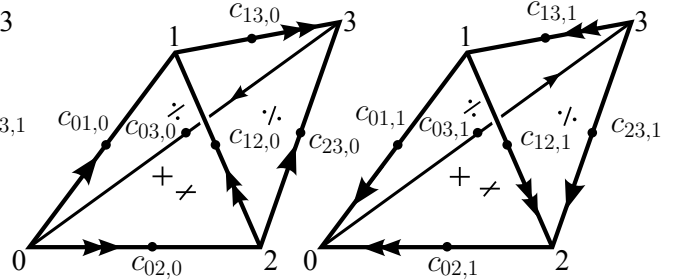
Figure 7. Oriented triangulation of the figure 8 knot sister. The signs indicate the non-trivial obstruction class.
