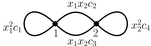
Figure 9. The diagonal action of (x_1, x_2) .
