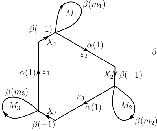
Figure 14. 3-cycle case.
