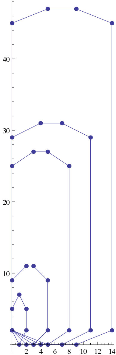
Figure 2: The Newton polygon of the twisted (inhomogeneous) recurrences for the knot 4_1 in (L, M^m) -space; note that the slopes appear jolted due to the use of (L, M^m) coordinates.
