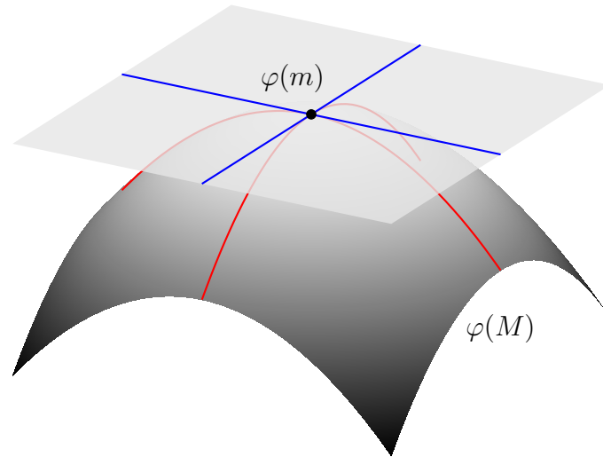
Figure 3.2: The 1-jet at m \in M of a smooth map \varphi : M \rightarrow F can be identified with the tangent plane of its image at \varphi(m) .
